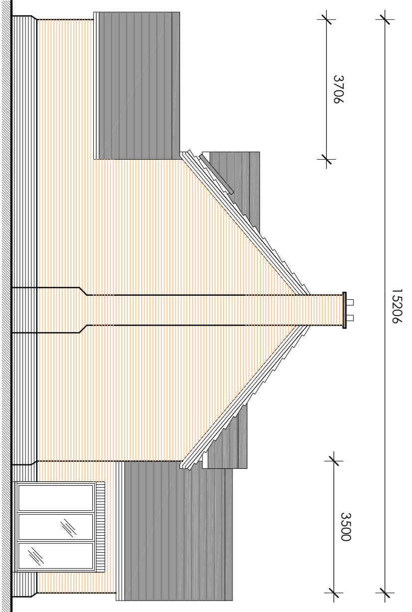
Side Elevation
