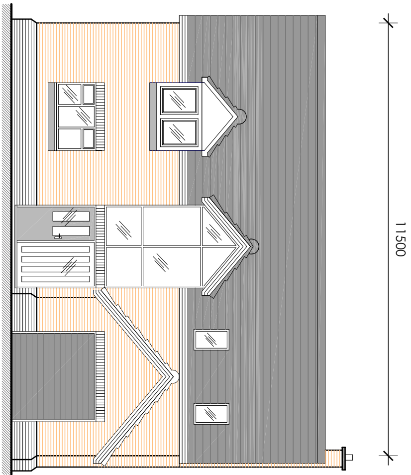
Front Elevation
