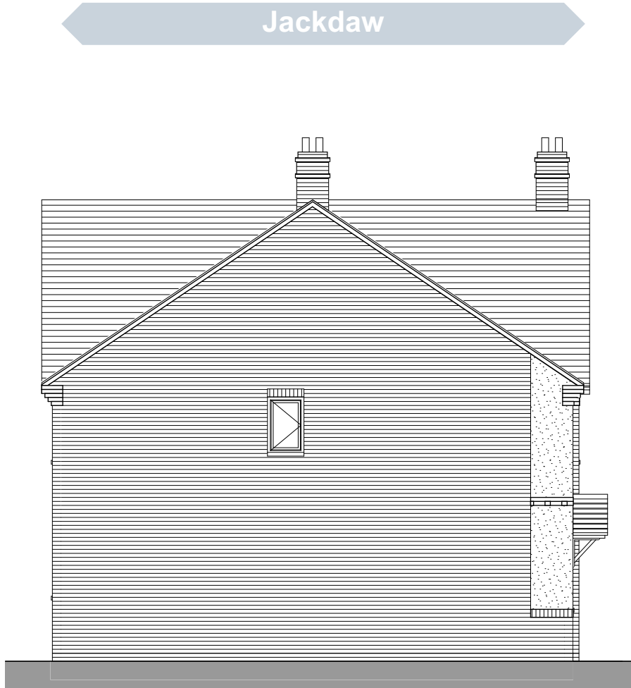
Side Elevation
