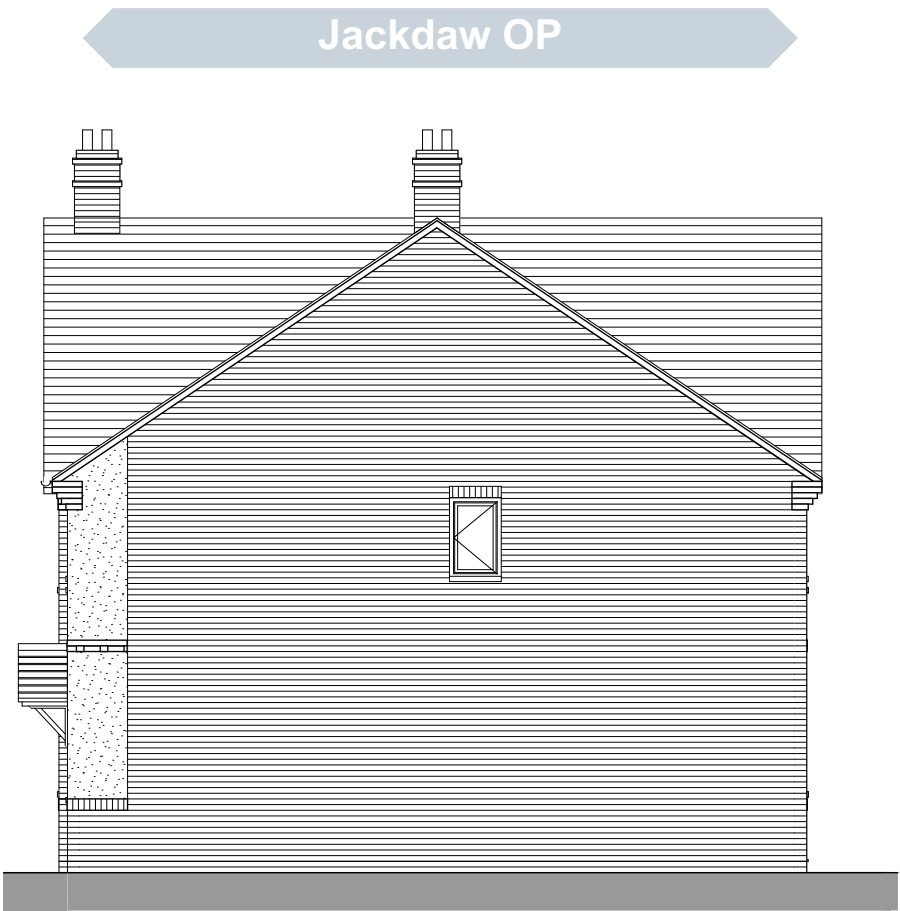
Side Elevation
