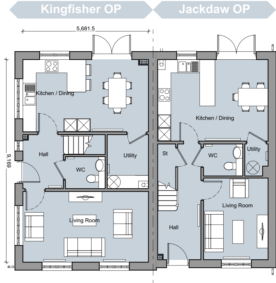
Ground Floor
