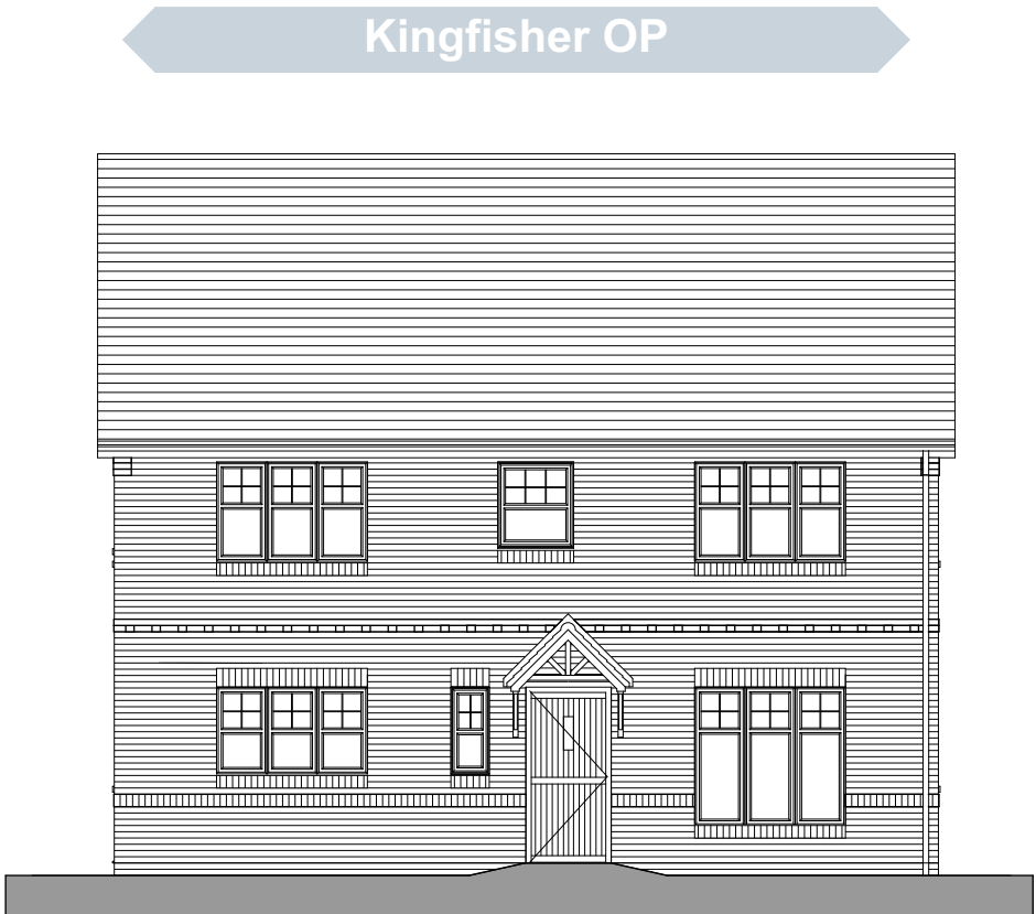
Side Elevation
