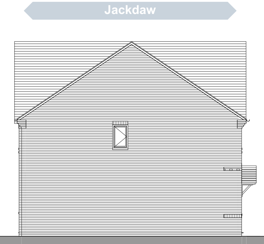
Side Elevation
