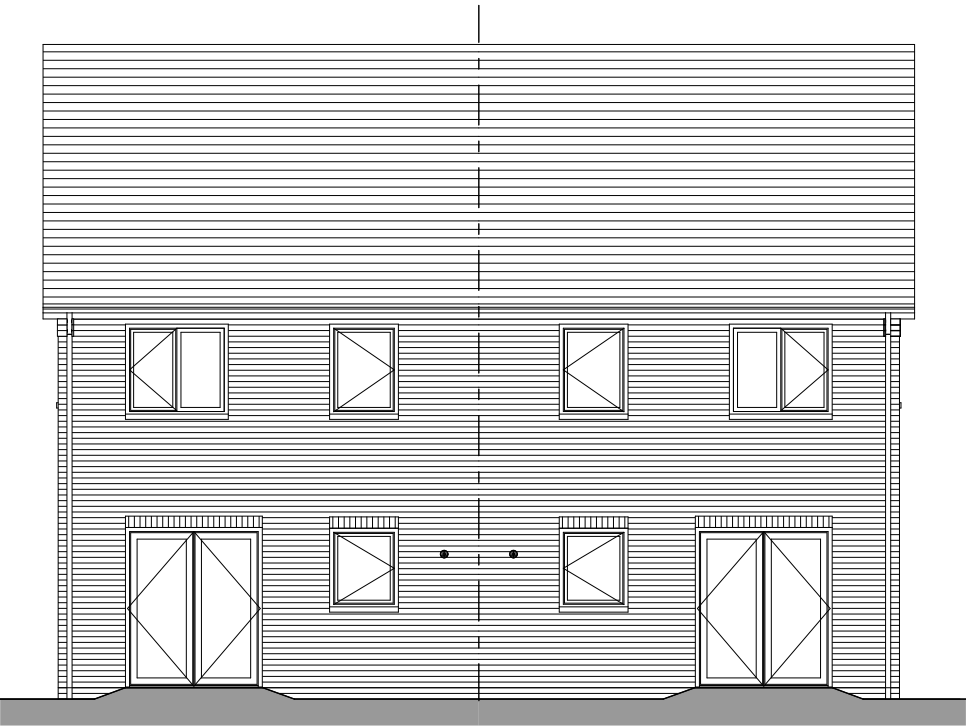
Rear Elevation
