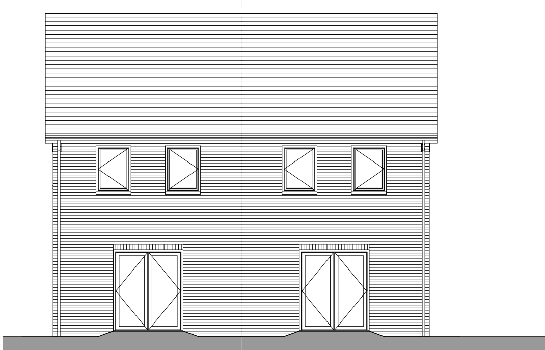
Rear Elevation
