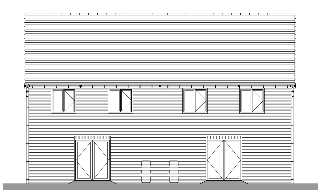
Rear Elevation
