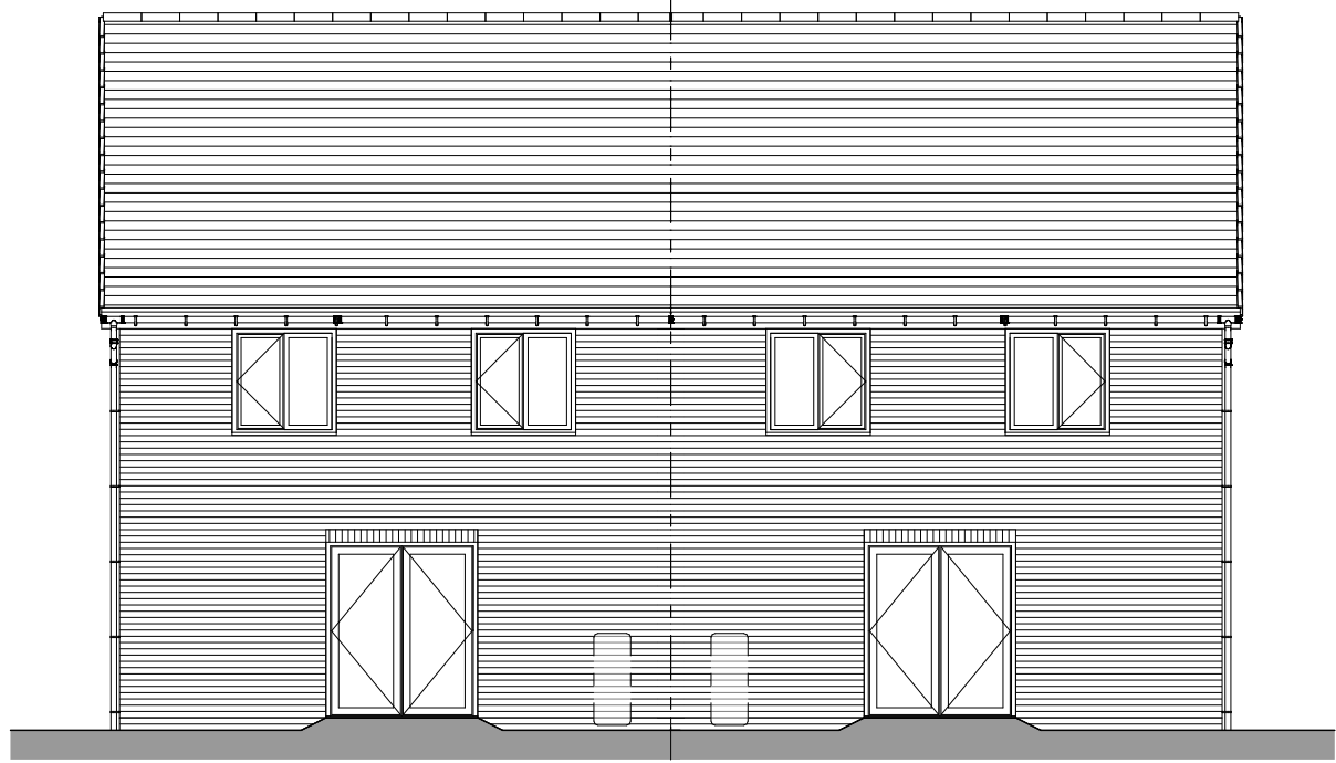
Rear Elevation
