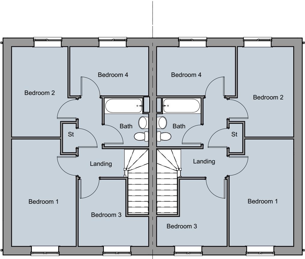
First Floor
