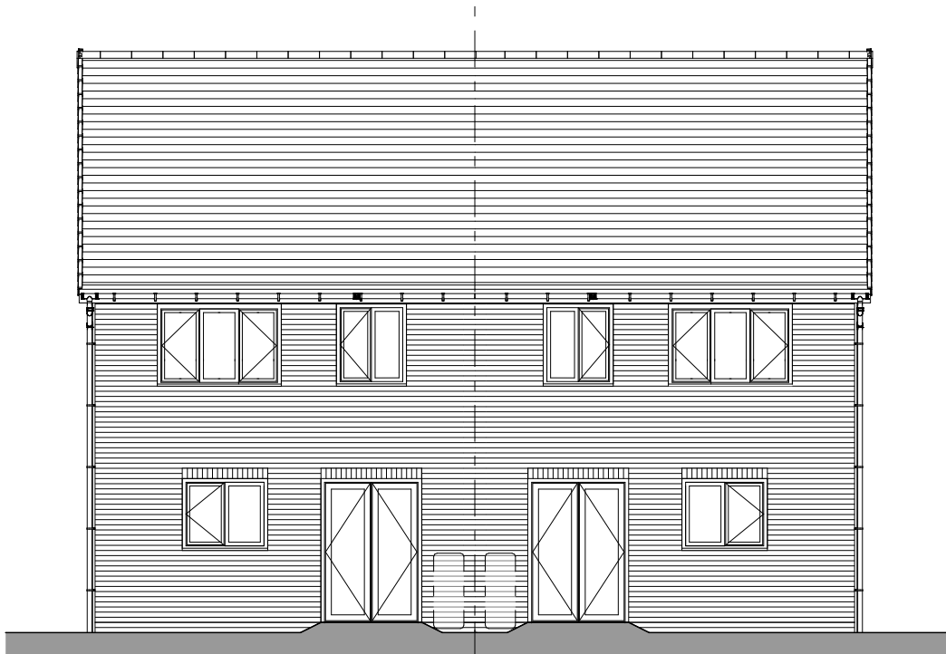
Rear Elevation
