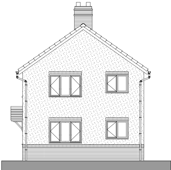
Side Elevation
