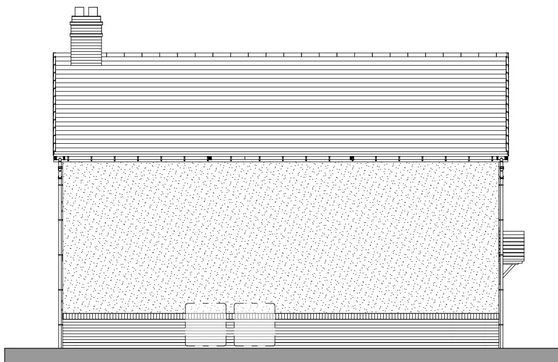
Rear Elevation
