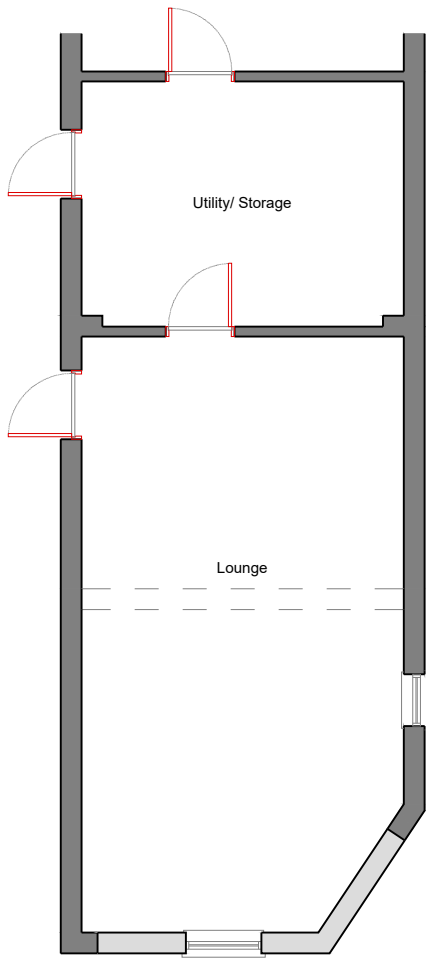
GROUND FLOOR PLAN SCALE - 1 : 100 Proposed
