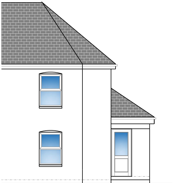
Proposed PART FRONT ELEVATION
