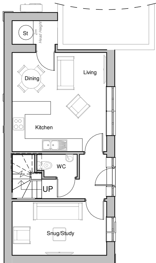
Proposed GF Plan - 1:100
