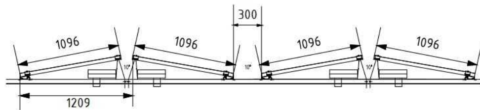
E/W FACING PANELS 10 DEGREE PITCH & 300mm SPACING
