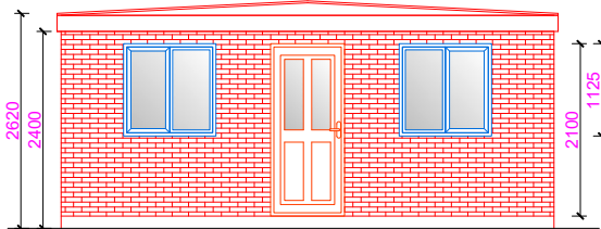
NORTH-EAST ELEVATION
