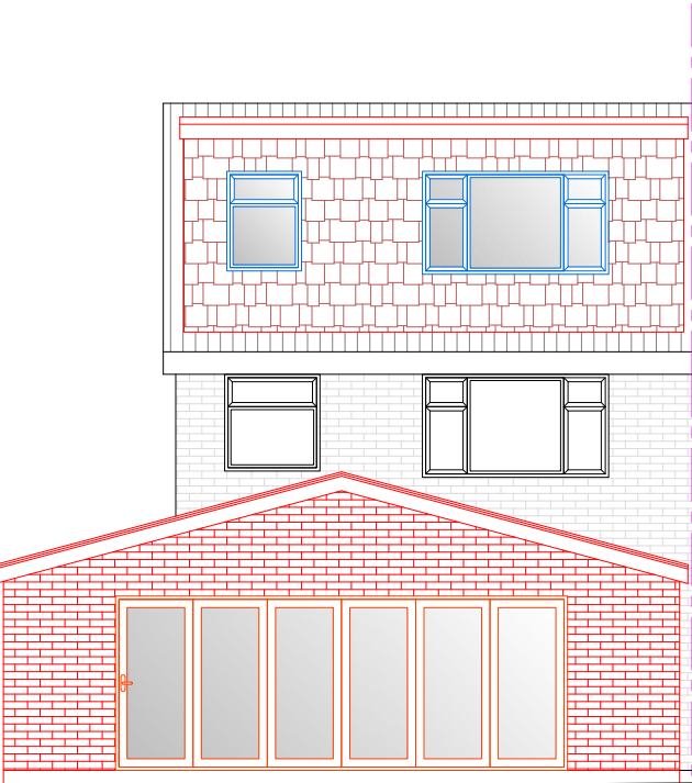
SOUTH-WEST ELEVATION
