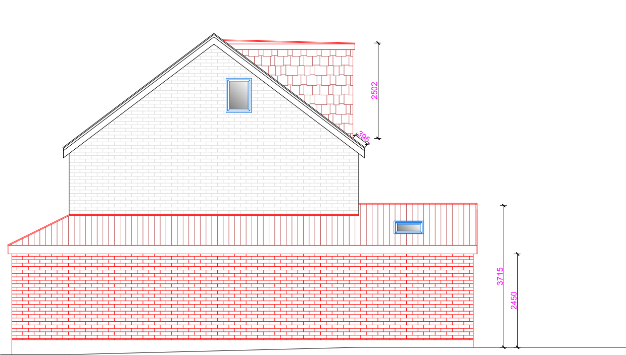
NORTH-WEST ELEVATION
