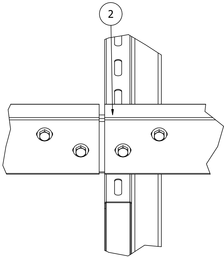
DETAIL VIEW J ( 1:4 )
