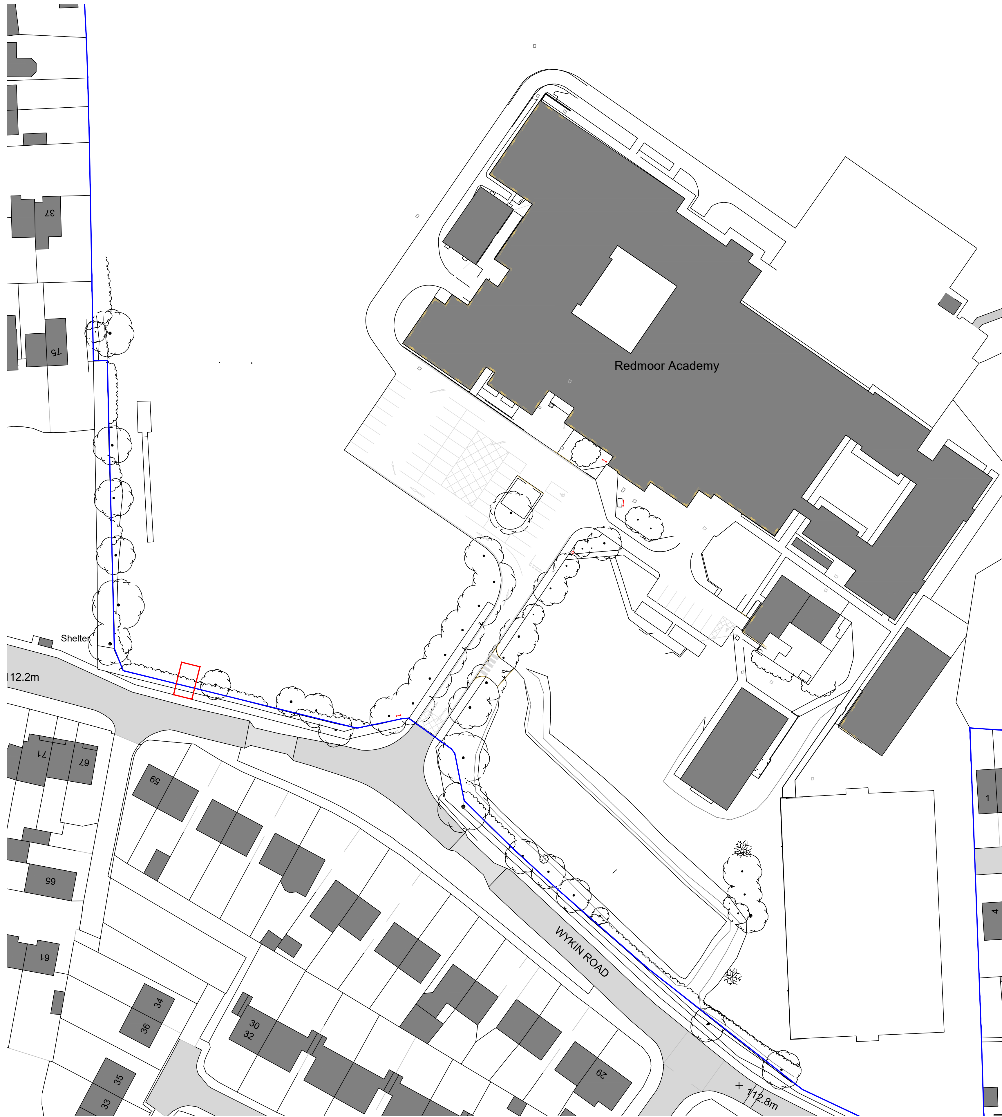
2 Site Block Plan (SCALE 1:500)
