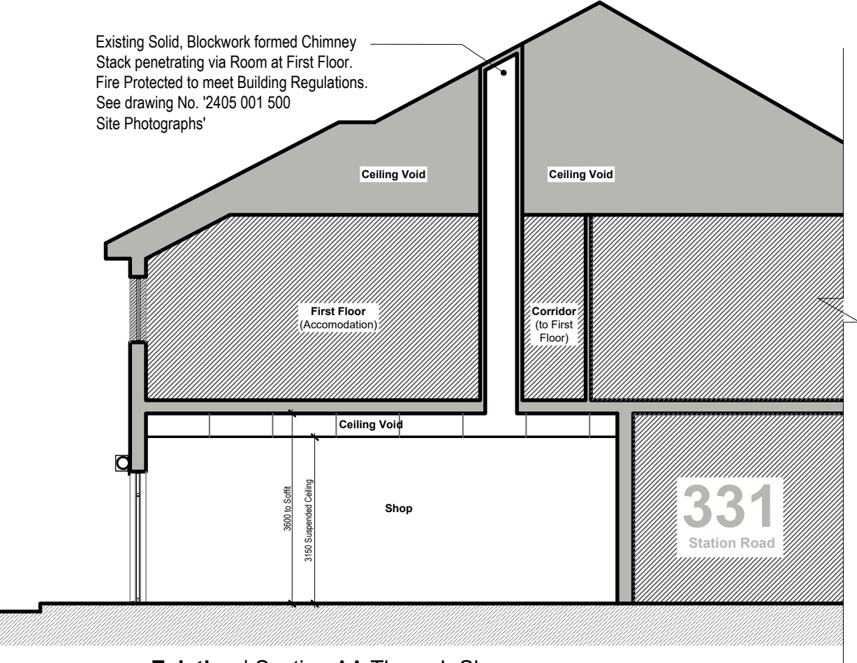
Existing | Section AA Through Shop
