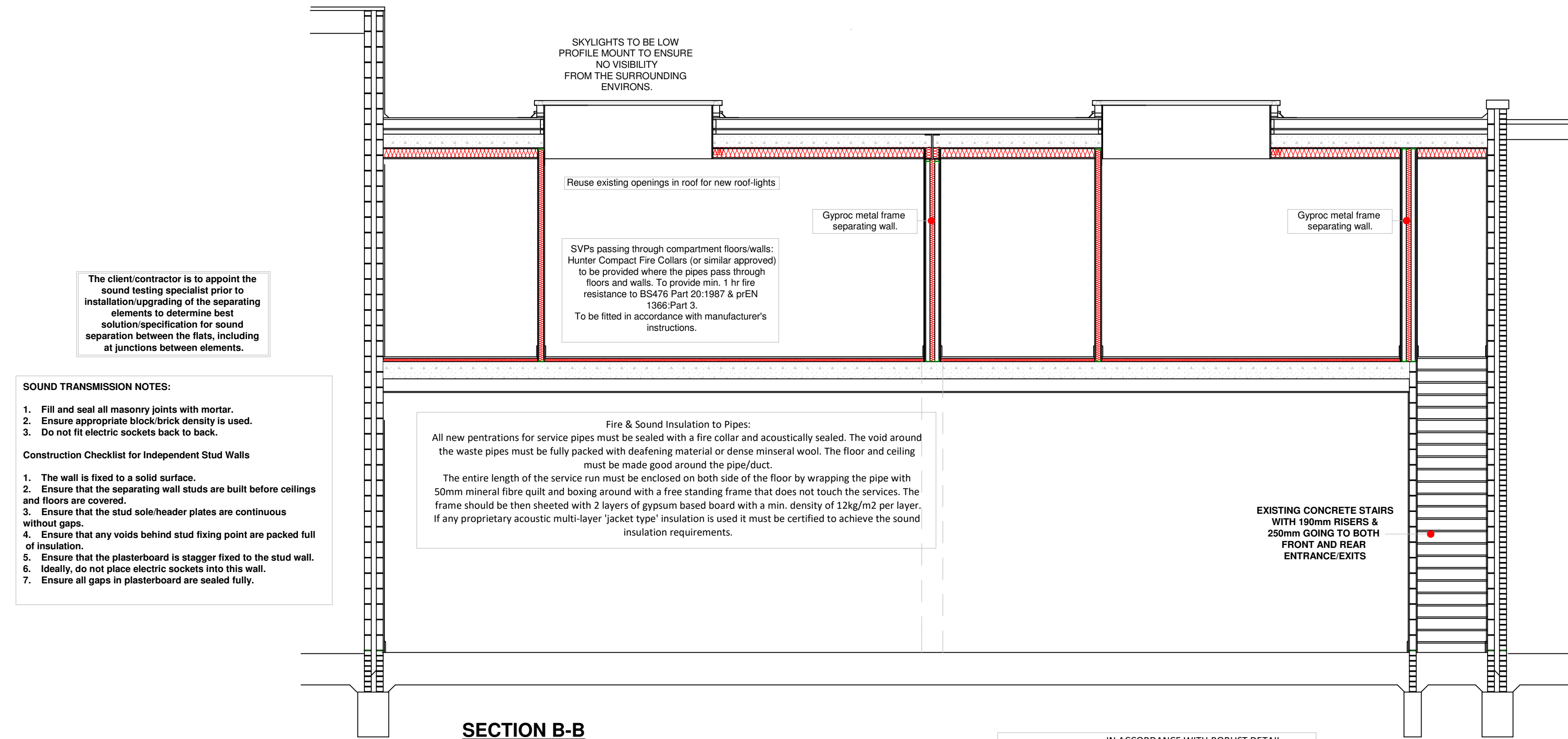
SECTION B-B
