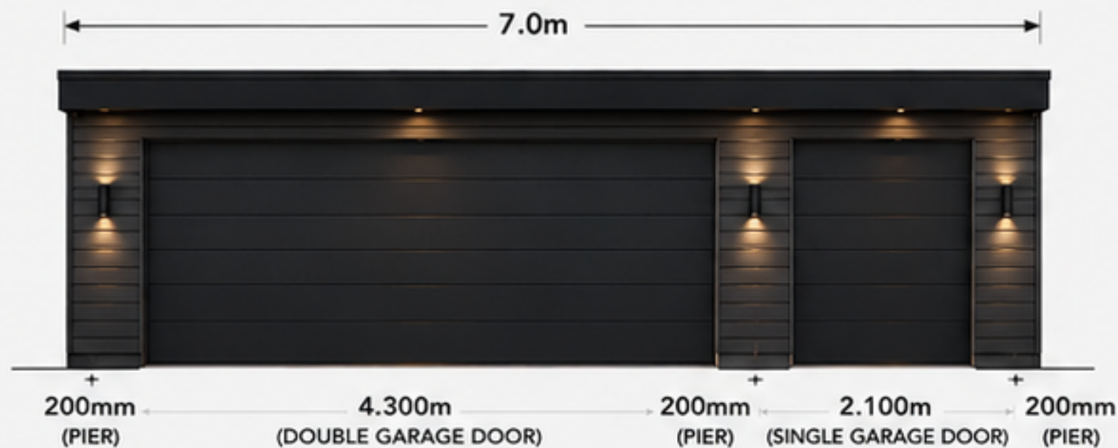
FRONT ELEVATION
