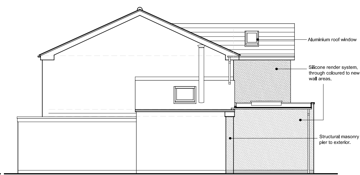
Side Elevation 1 South West
