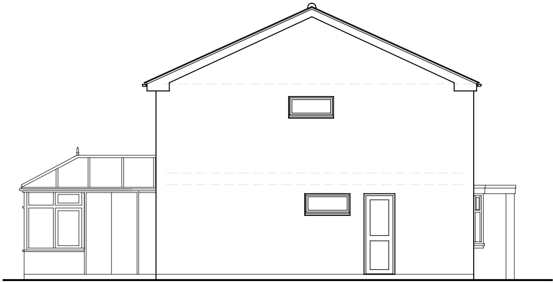
Side Elevation 2 North East
