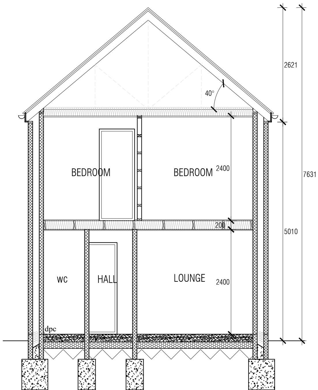
PROPOSED SECTION A-A PLOT 3
