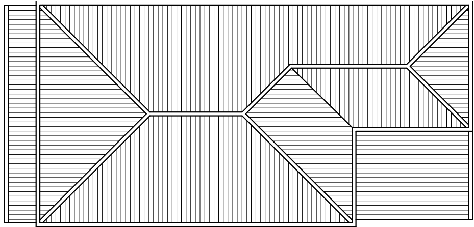
PROPOSED ROOF PLAN.PLOT 3
