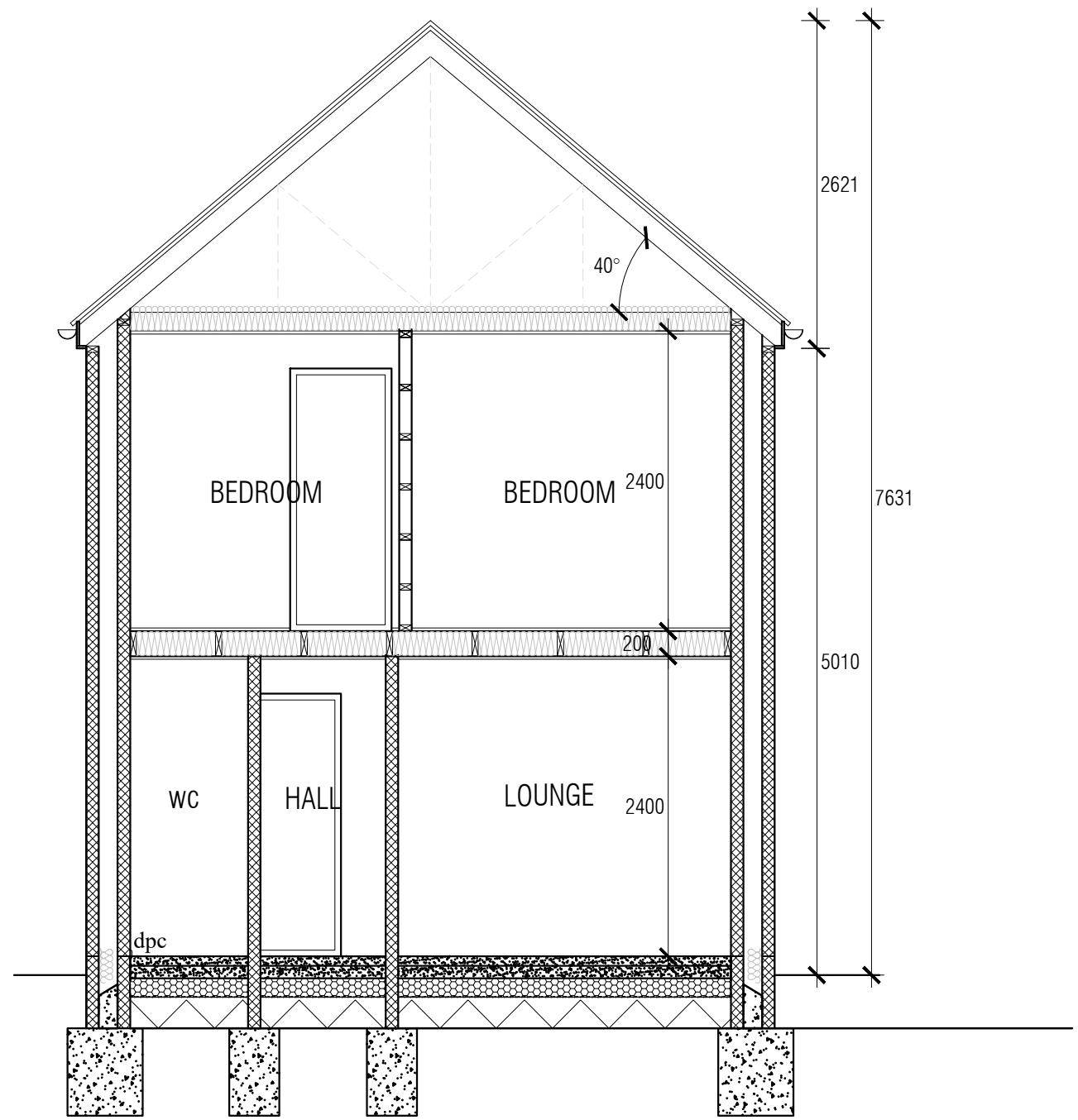
PROPOSED SECTION A-A PLOT 2
