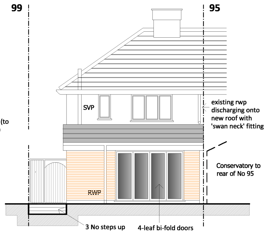
PROPOSED Rear Elevation - North Facing
