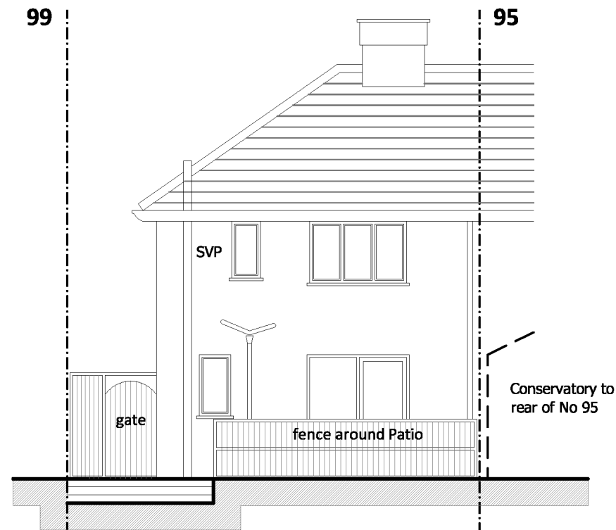
Existing Rear Elevation - North Facing
