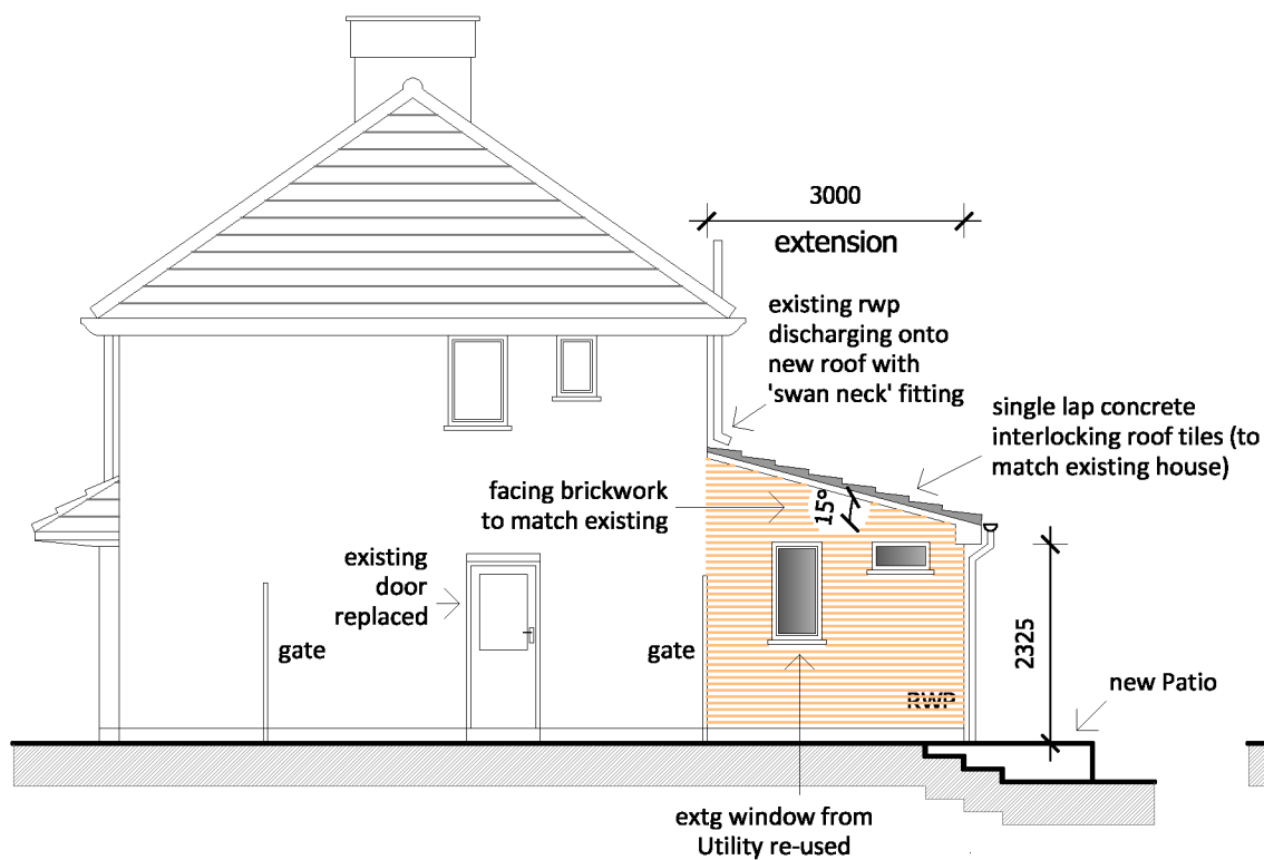
PROPOSED Side Elevation - Facing No 99
