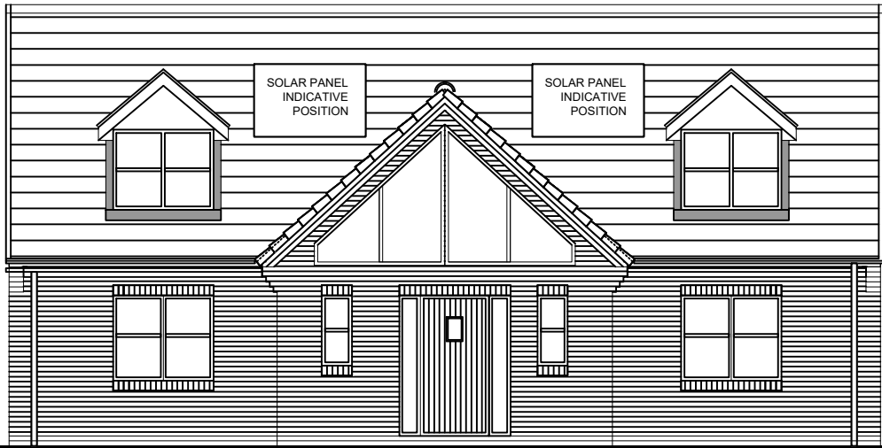
FRONT ELEVATION
