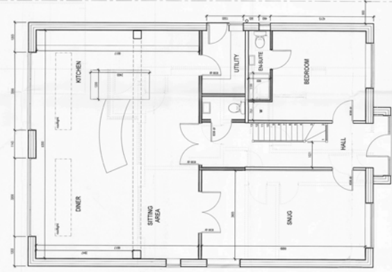
PROPOSED GROUND FLOOR PLAN Scale 1:50
