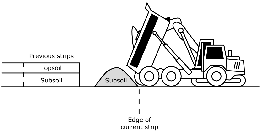
Figure D.2a: Soil replacement with excavators - dump trucks: Subsoil layer.
