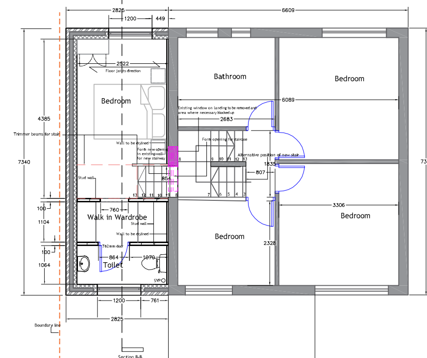
Proposed Plans and Elevations
