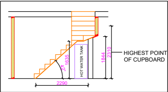
STAIR SECTION
