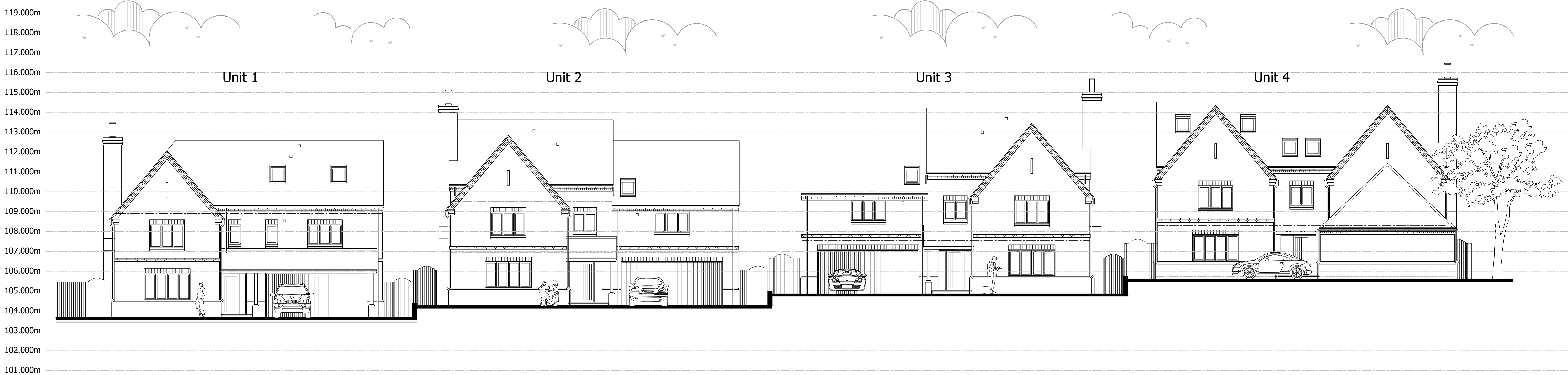
Illustrative Site Section - Units 1 to 4 Scale 1:100
