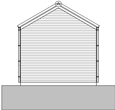
Rear Elevation. 1 : 100
