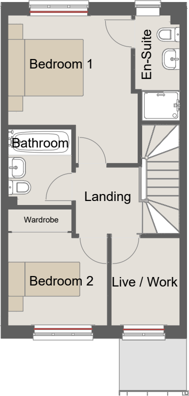
First Floor 1 : 100
