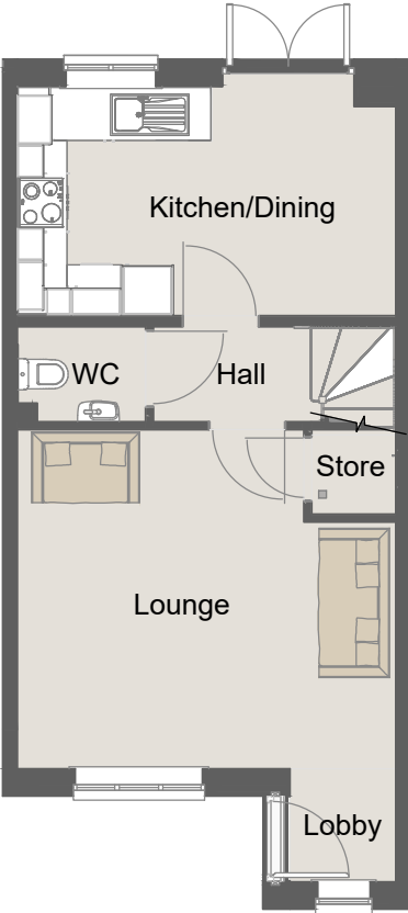
Ground Floor 1 : 100
