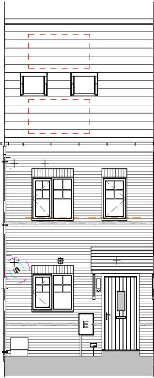
Front Elevation 1 : 100
