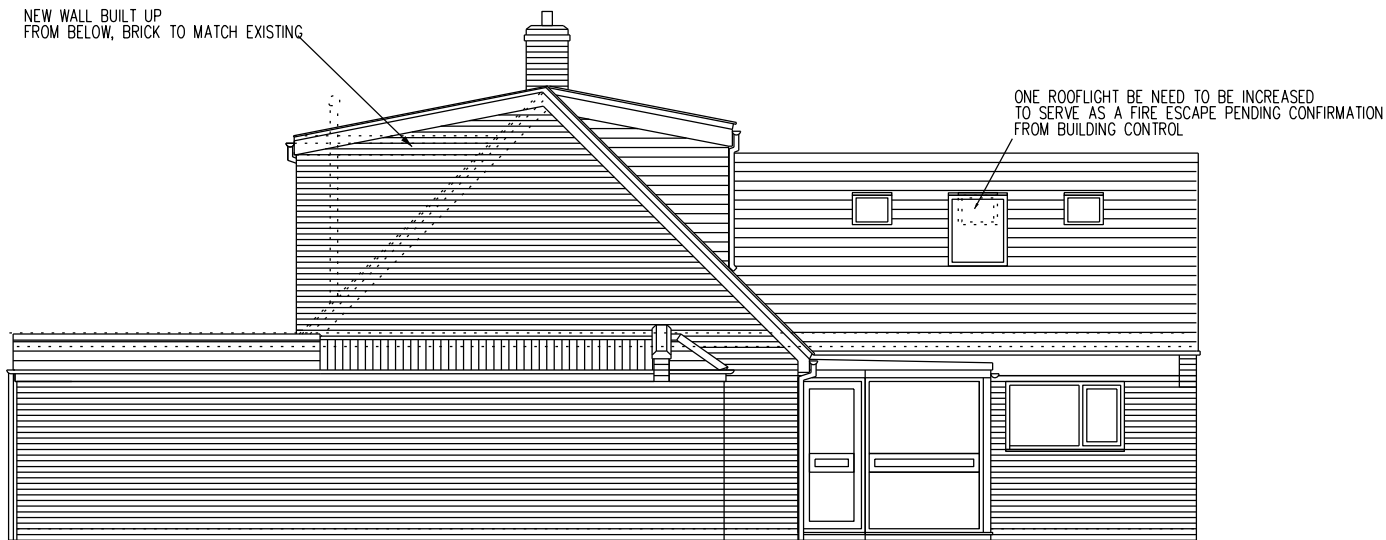
SIDE ELEVATION PROPOSED
