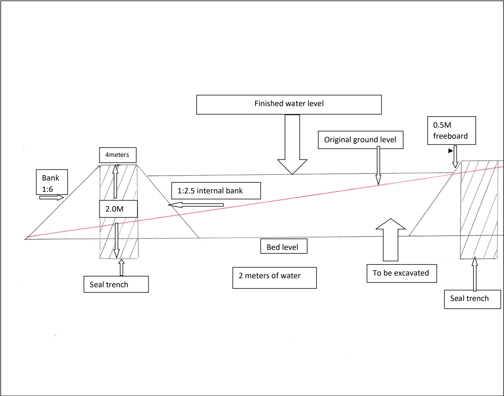
Proposed Lake cross section. Not to scale
