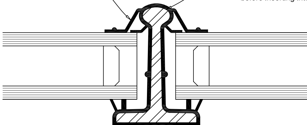
No.7 'Heritage' Lead Covered Steel Glazing Bar with 28mm infill
