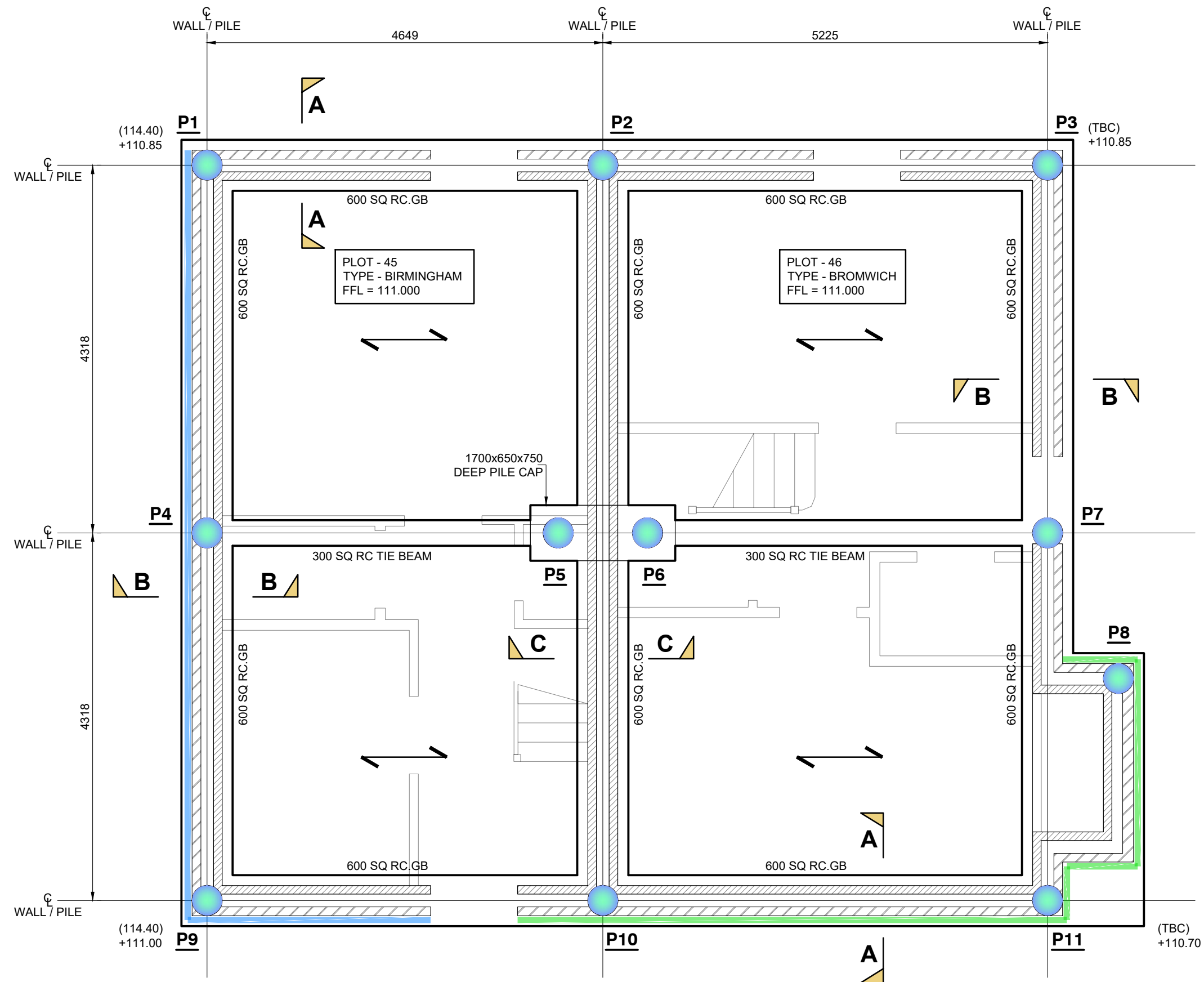
FOUNDATION LAYOUT INDICATION GROUND FLOOR SLAB (PLOT 45-46) (Scale 1:50)
