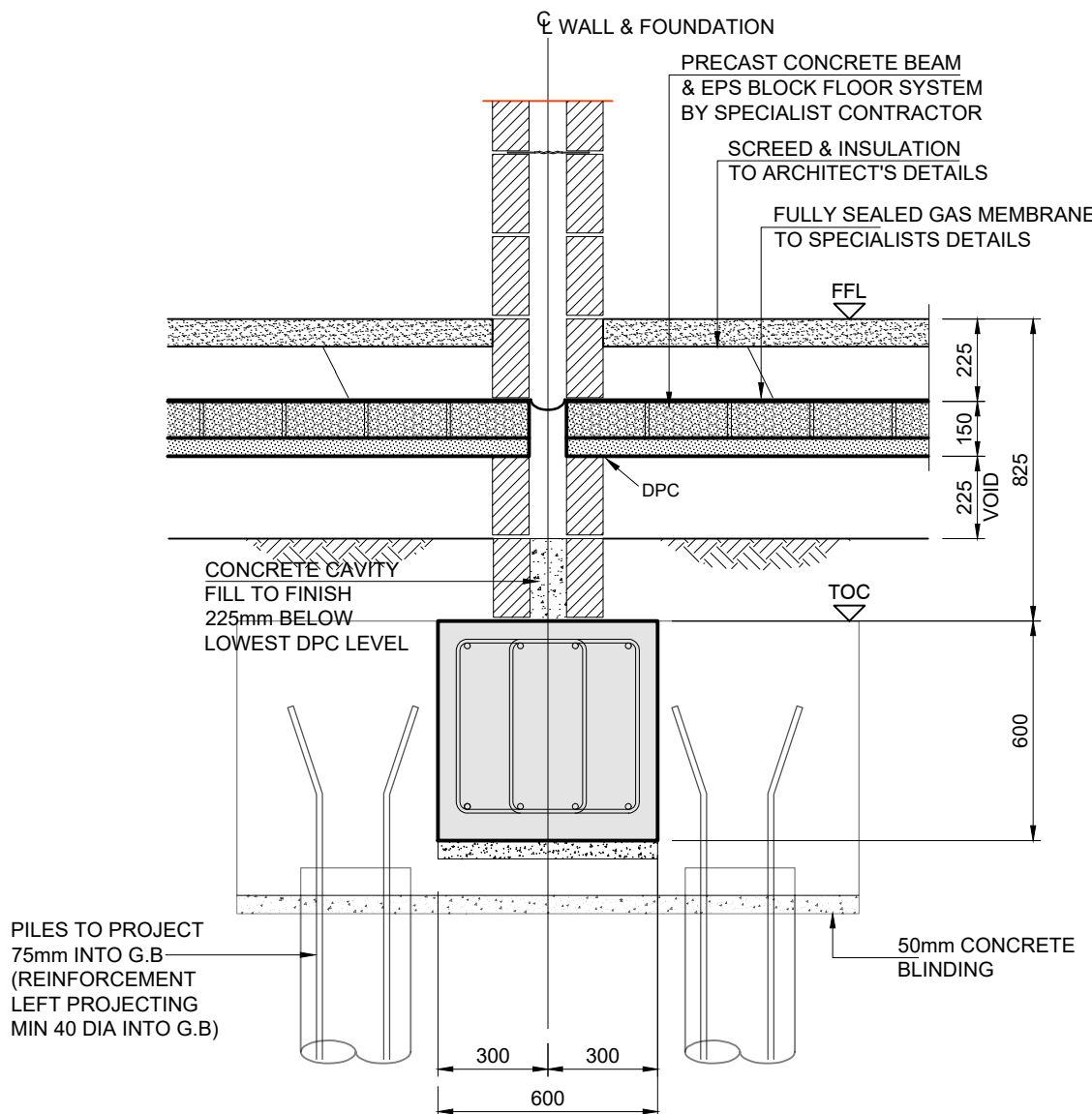
SECTION C-C SCALE 1:20
