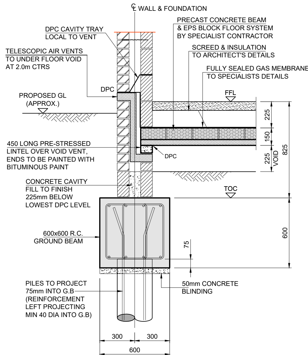
SECTION B-B SCALE 1:20
