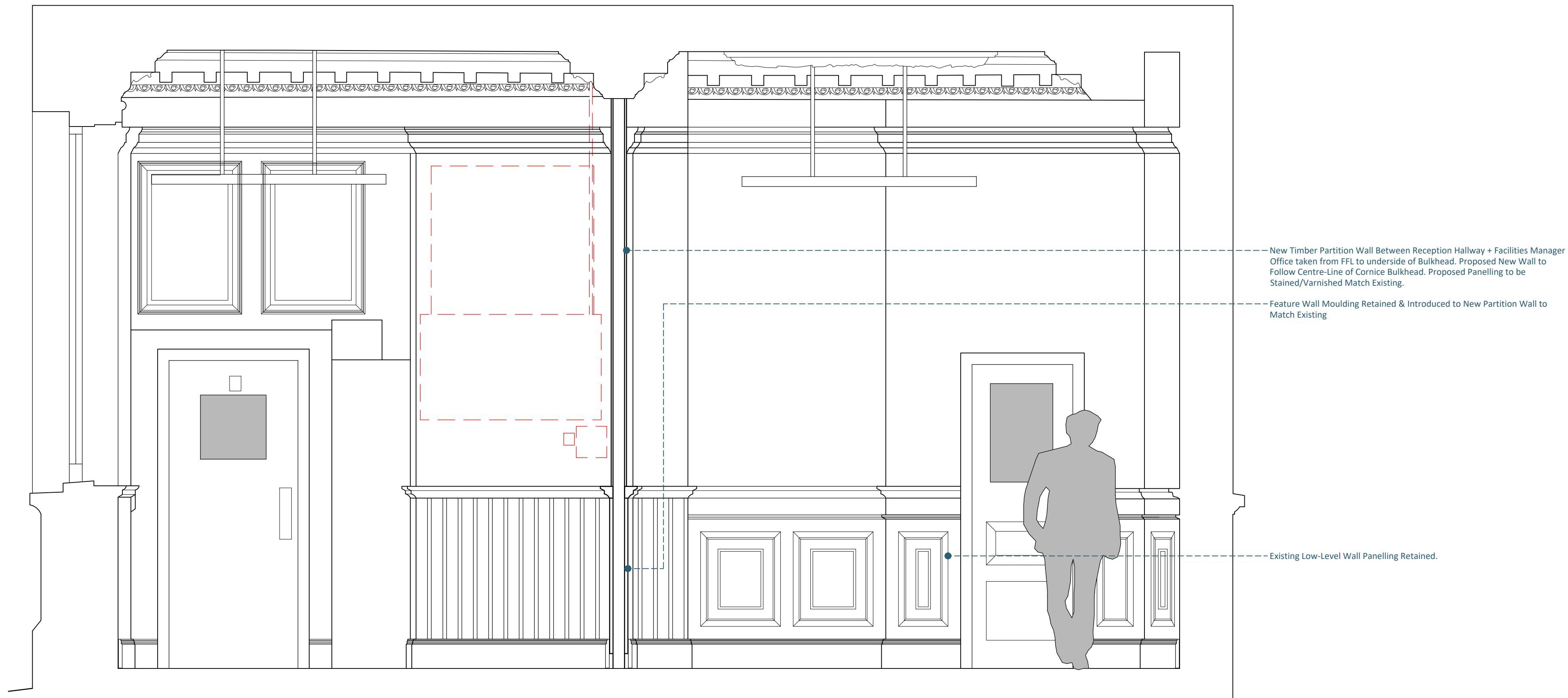
Proposed Internal Elevation 4 Scale 1:20
