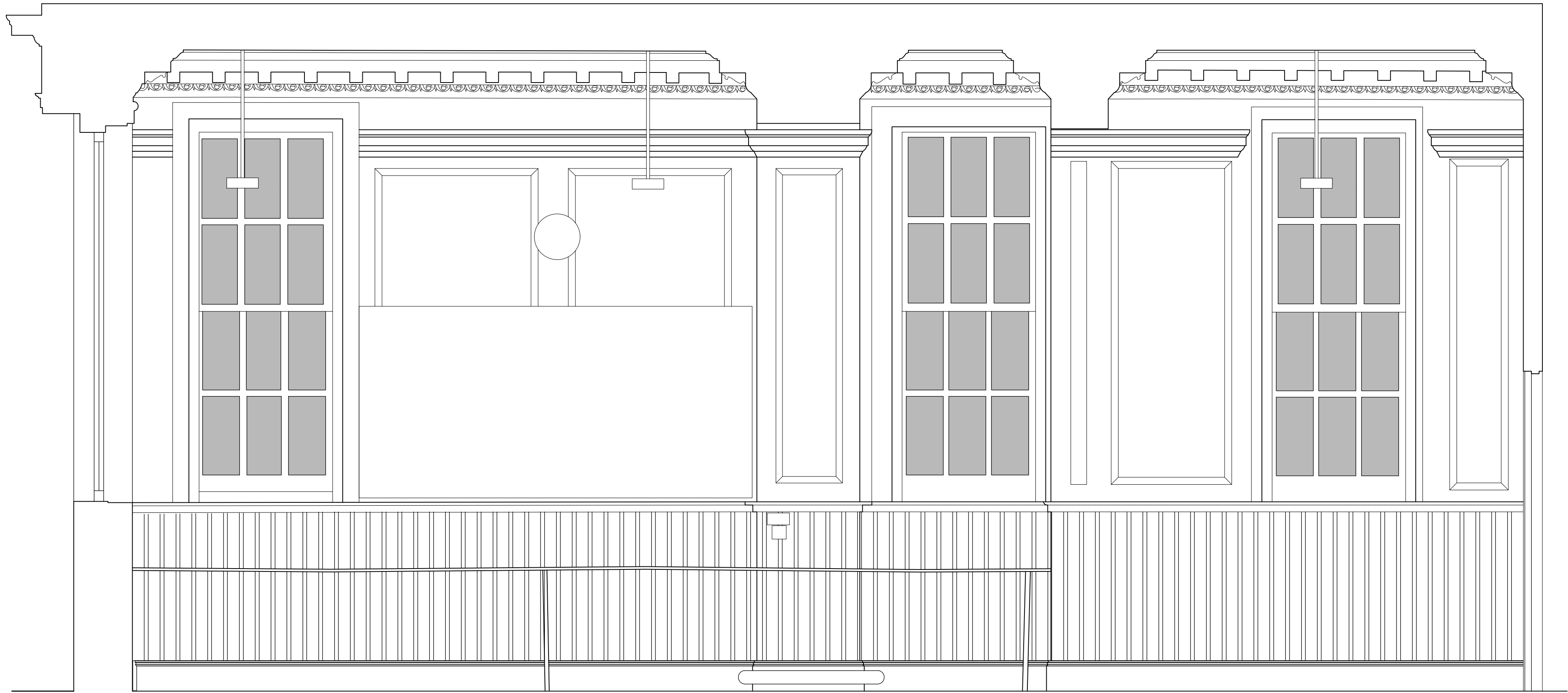
Existing Internal Elevation 1 Scale 1:20
