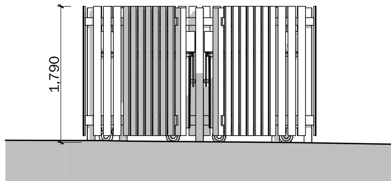
Elevation to North
