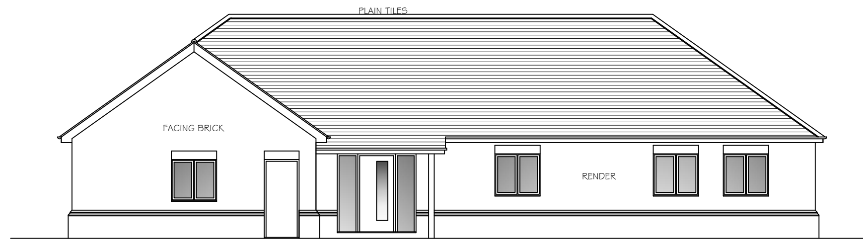
FRONT
