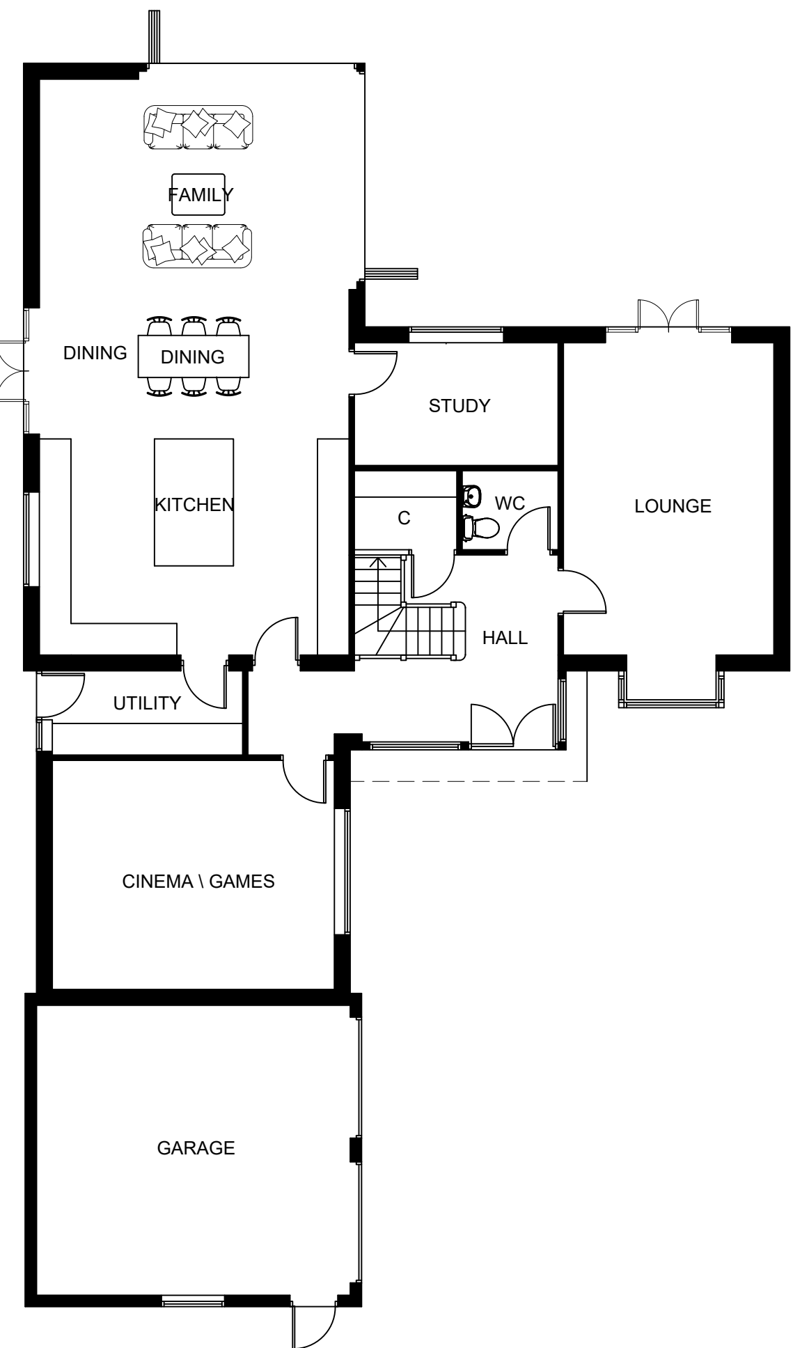
GROUND: UNIT 1
