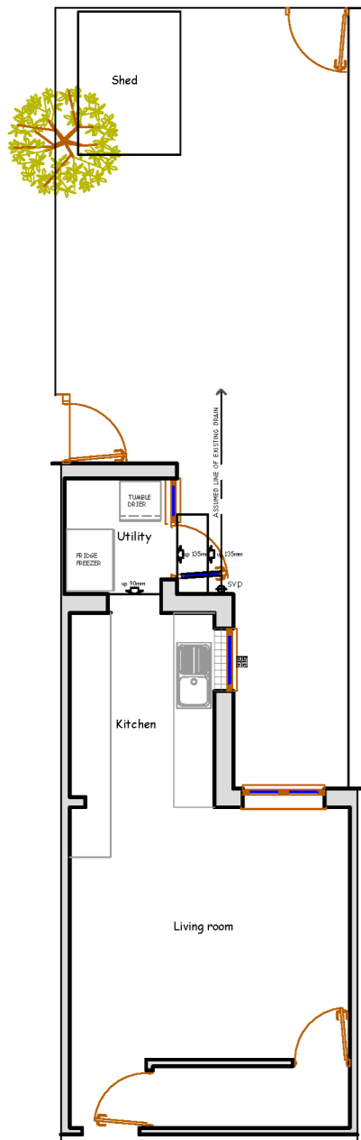
Existing Ground Floor Plan 1:100
