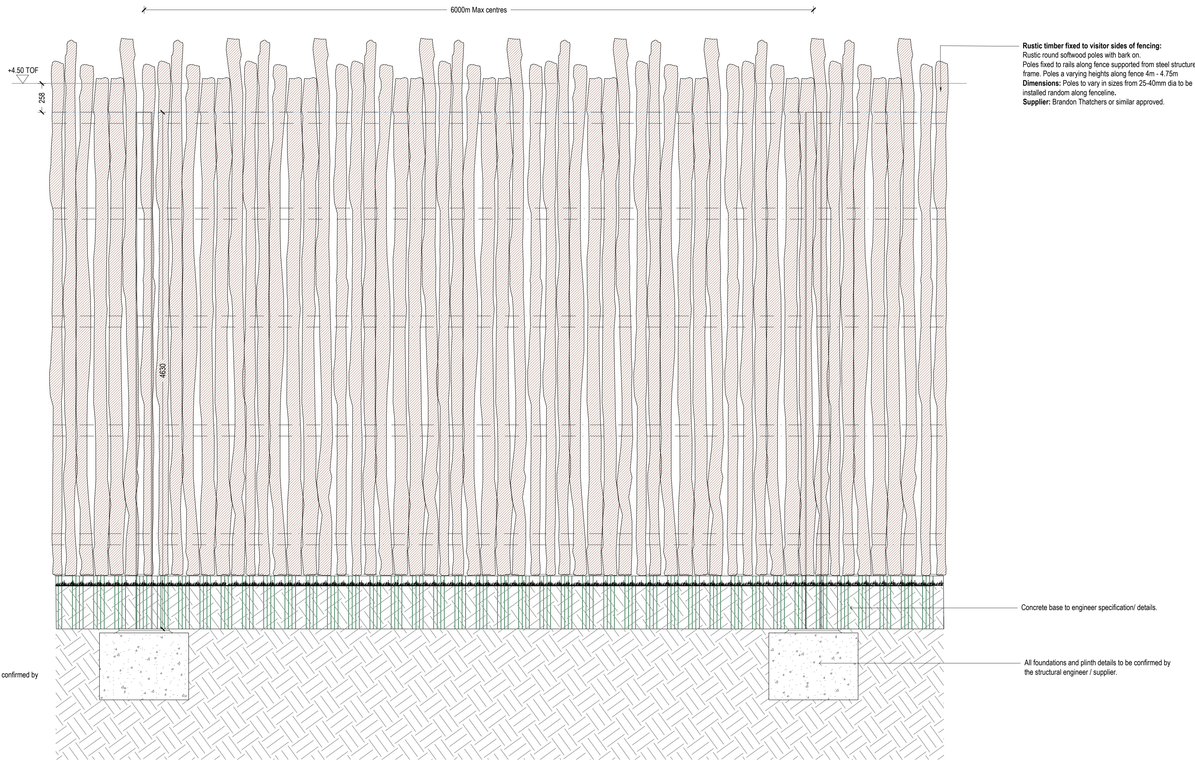
F2A 4.5m High visitor facing timber cladding elevation
