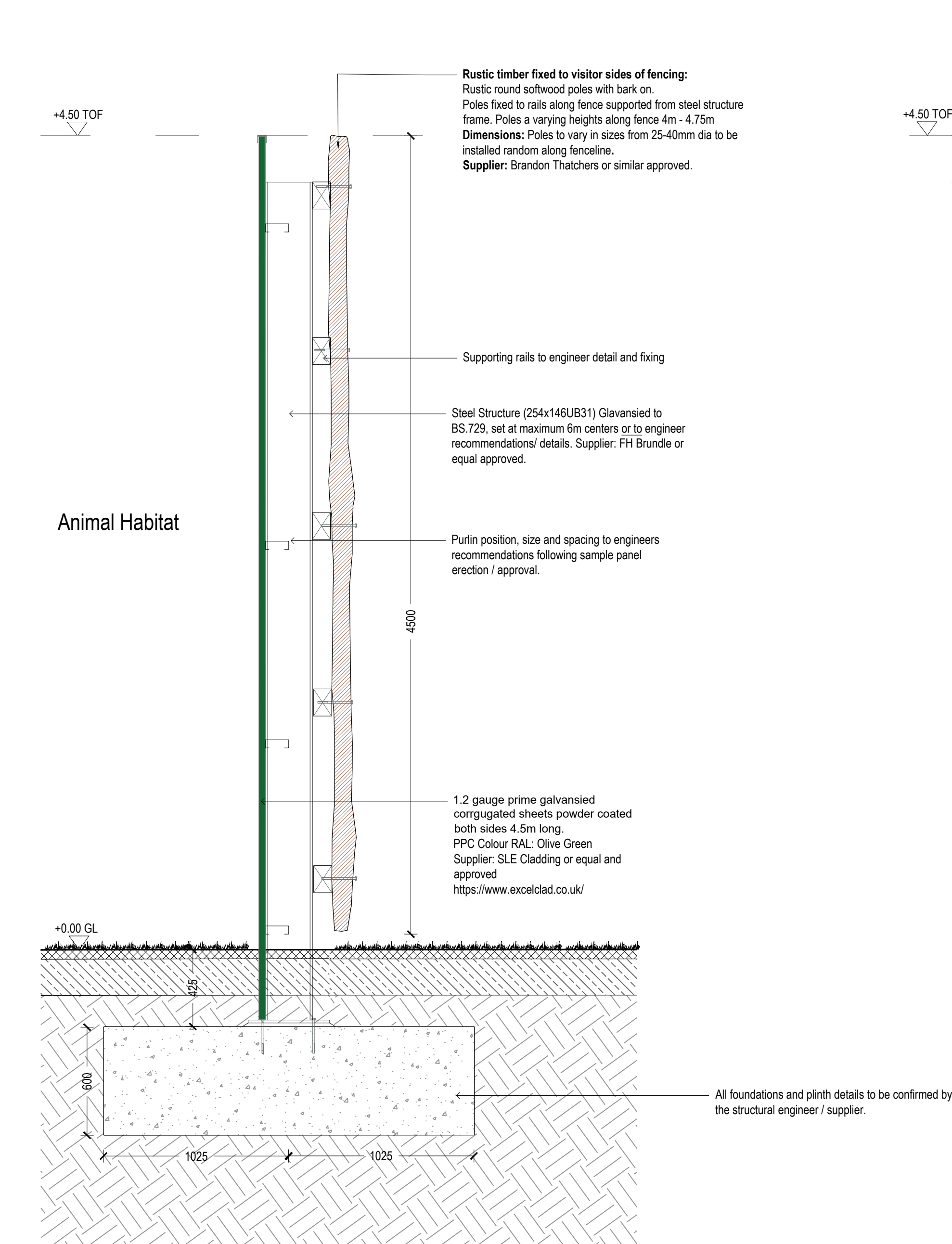
F2A Typical 4.5m High Steel Enclosure fence detail
