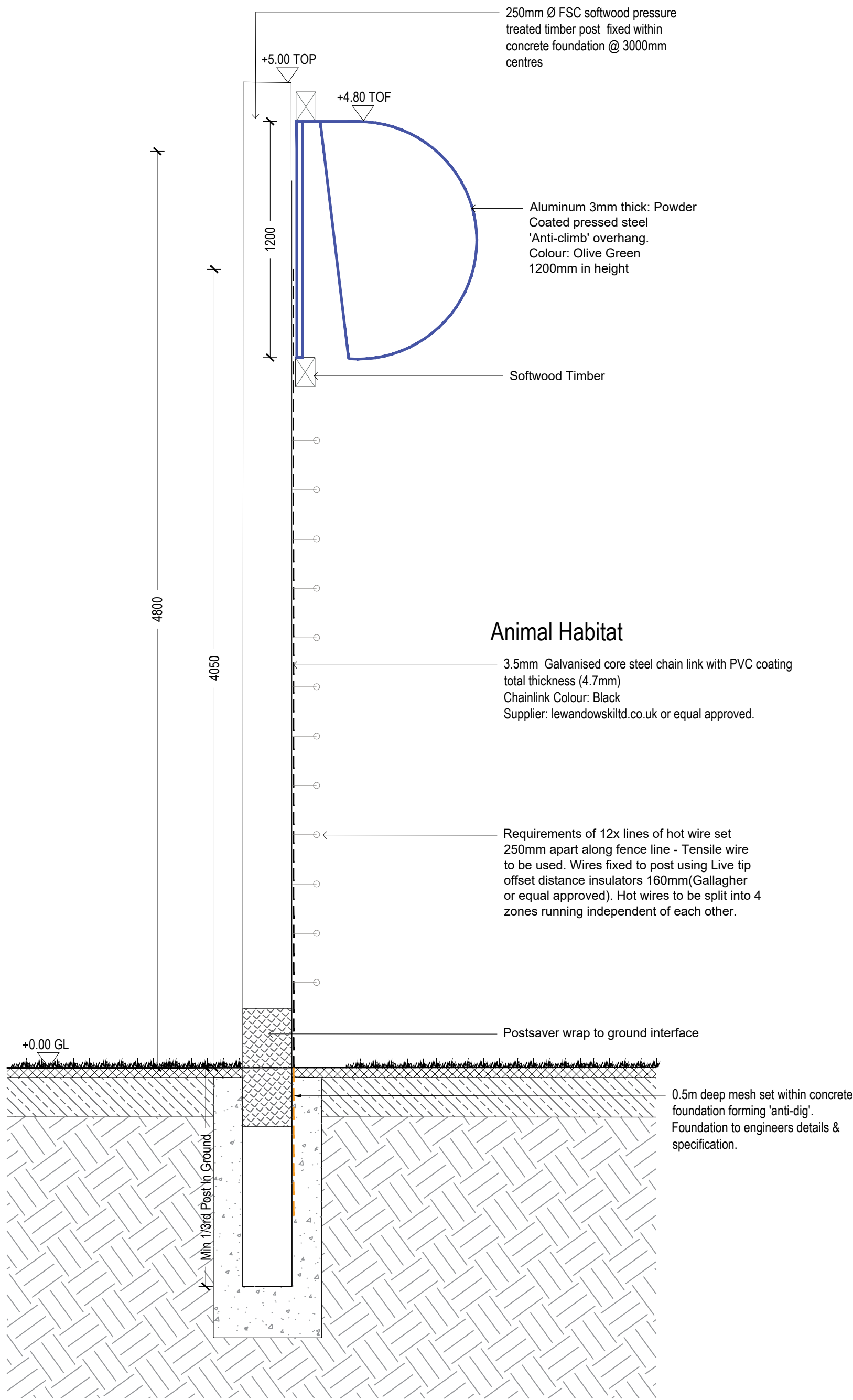
F1 4.5m High fence with Timber post, chainlink and antilimb
