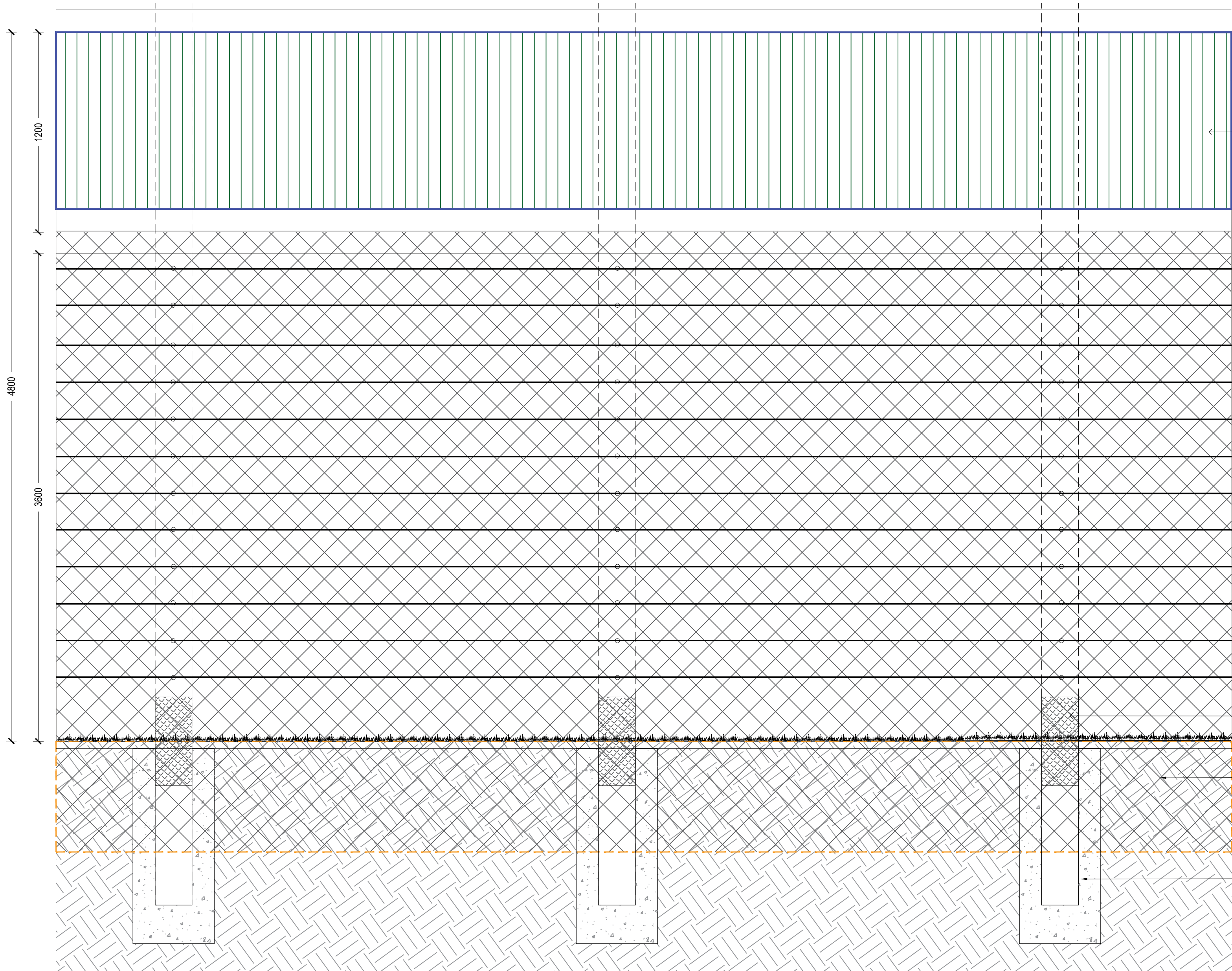
F1 4.5m High fence with Timber post, chainlink and antilimb Elevation
