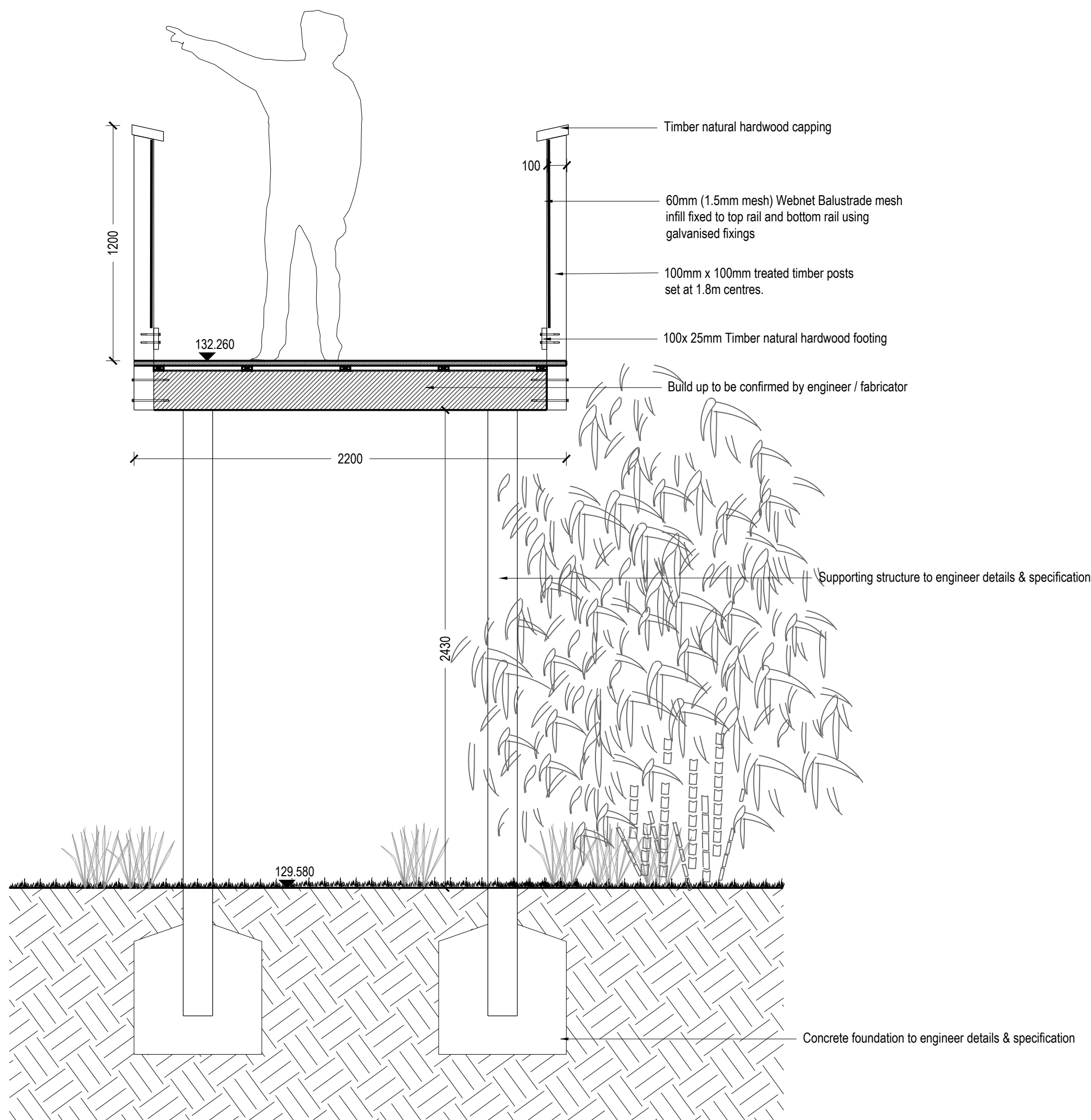
CROSS SECTION - through mid level boardwalk
