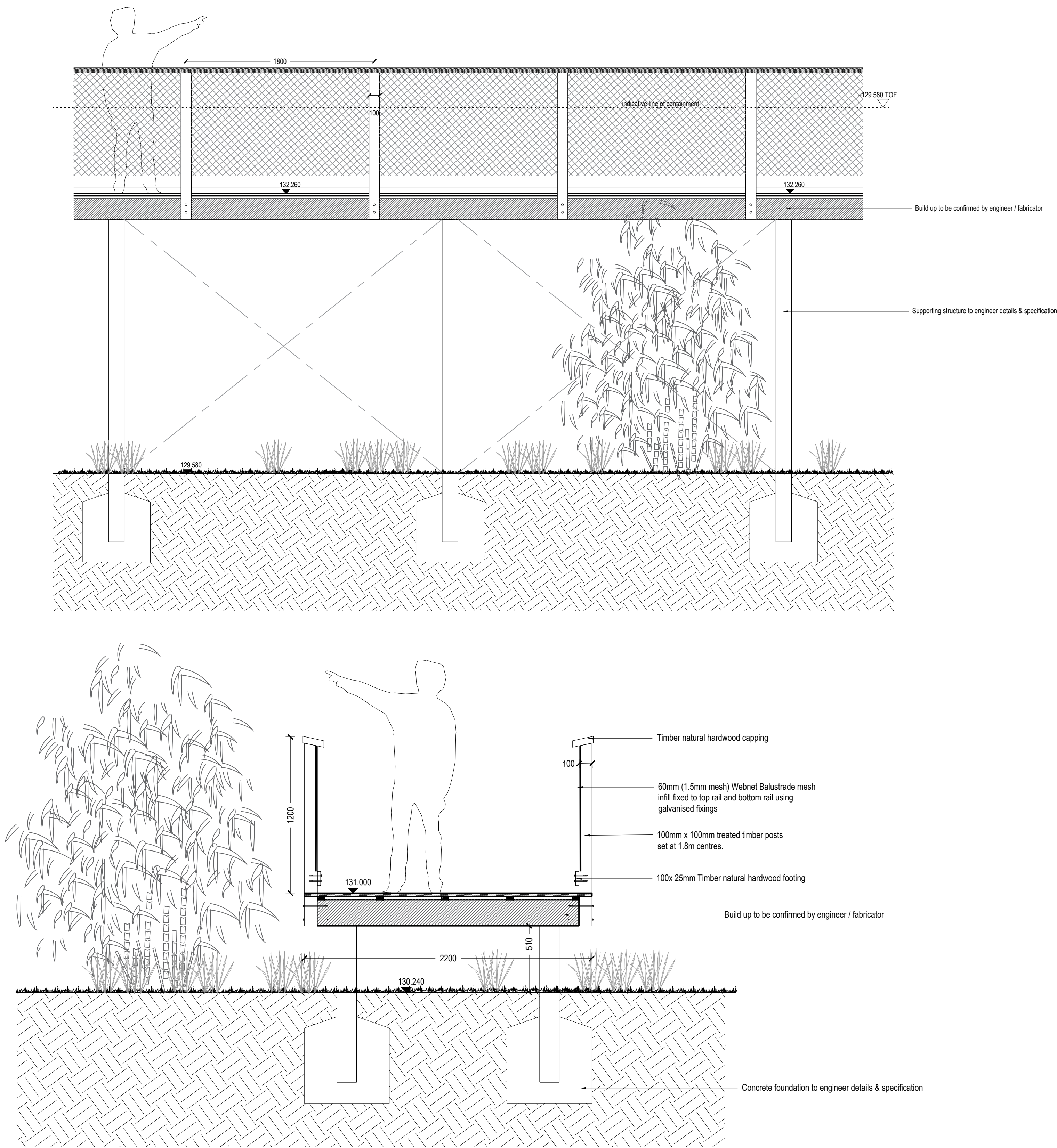
CROSS SECTION - through low level boardwalk
