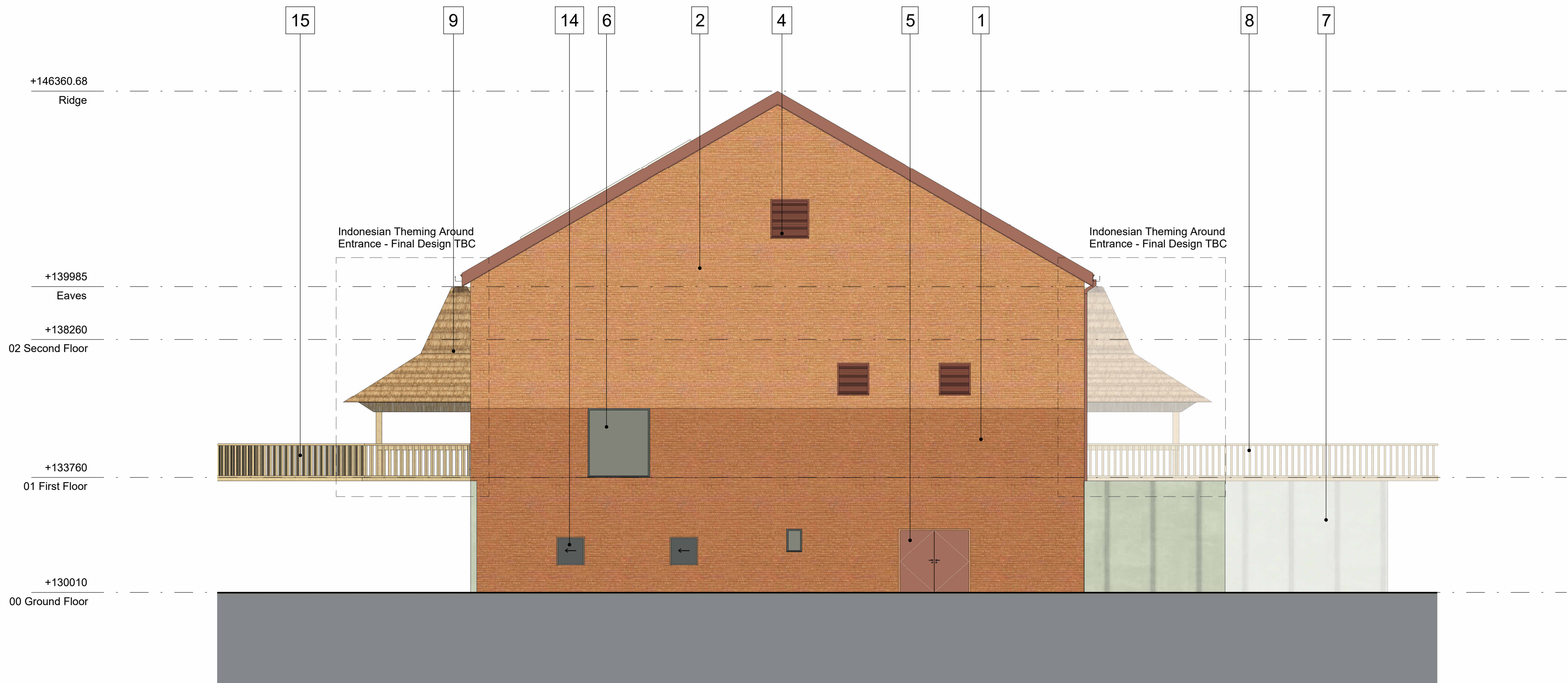
Elevation D: East - Orangutan Habitat Building Scale: 1 : 100
