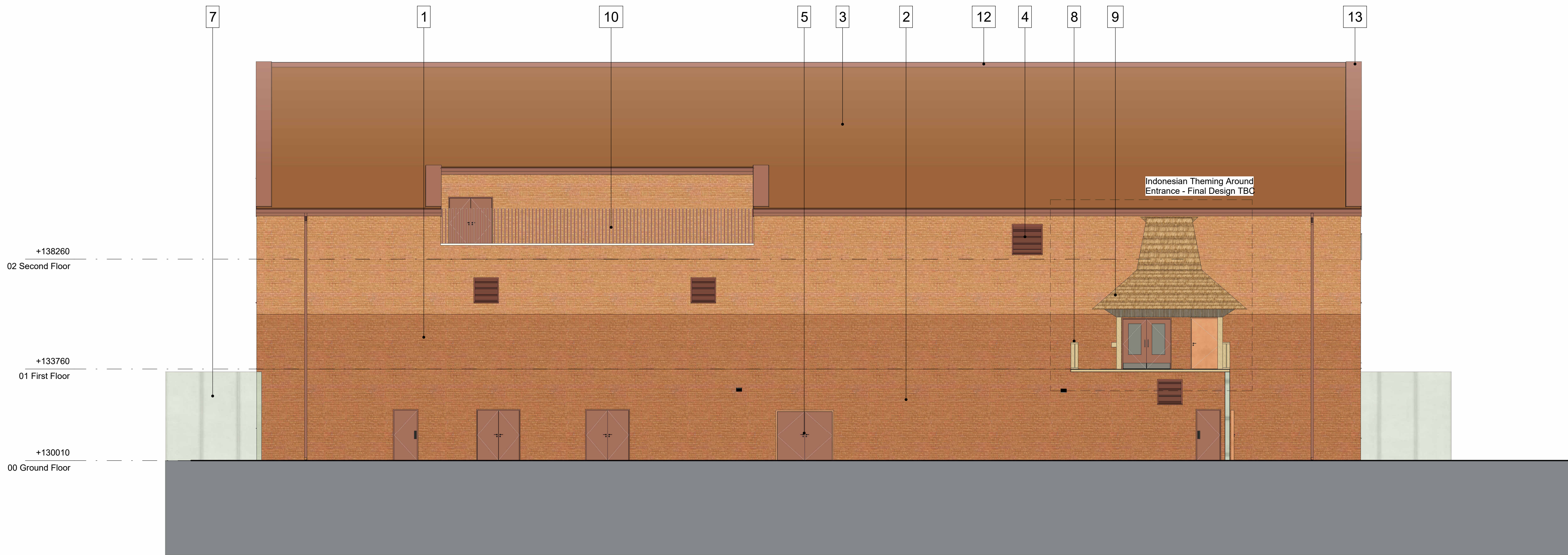
Elevation C: North - Orangutan Habitat Building Scale: 1 : 100
