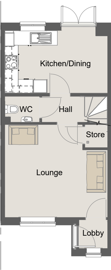
Ground Floor 1 : 100
